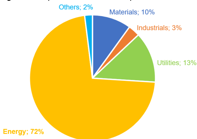
Fig. 2 Intensity of financed emissions by investment sector
