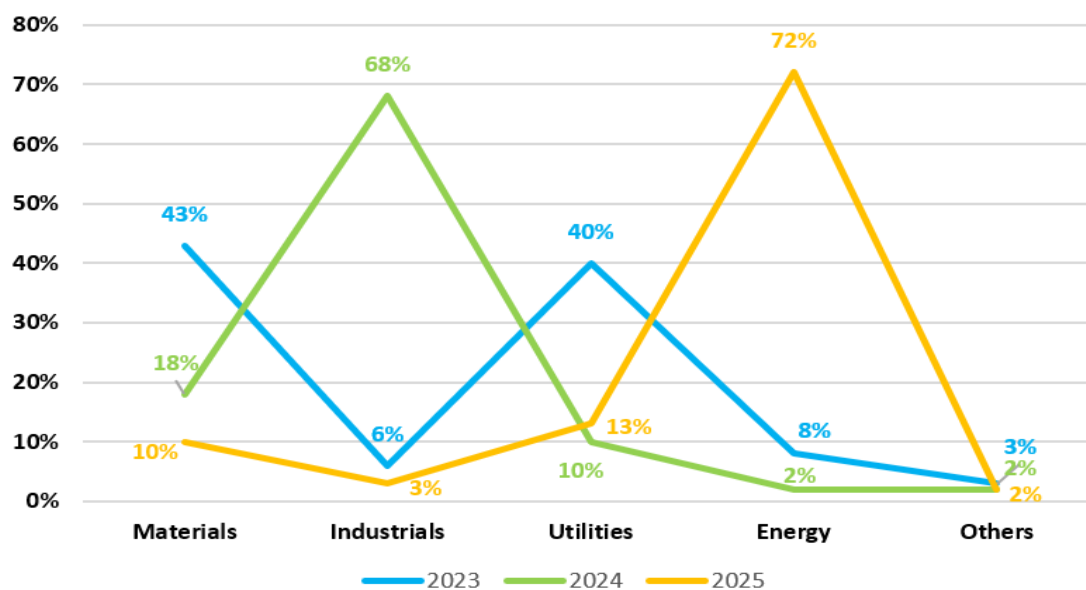
Fig. 1 Absolute carbon footprint by investment sector, 2023-2025
